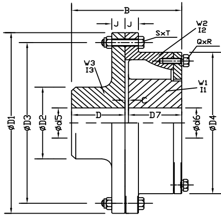
PCI SHAFT TO SHAFT RIGID HALF / FLEX HALF
